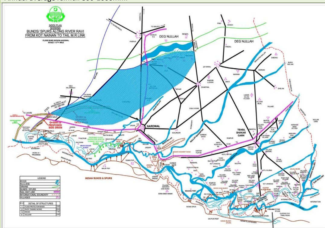
Figure 1: Lay Out of All Flood Bunds on River Ravi and its Tributaries in District Narowal
